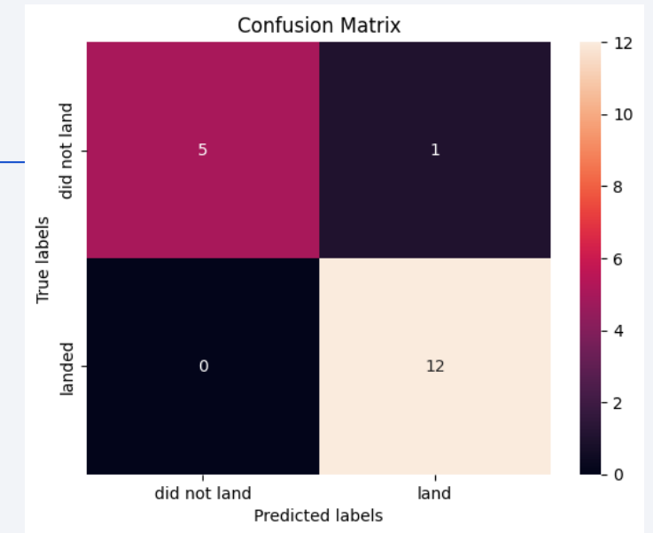
Decision Tree confusion matrix
