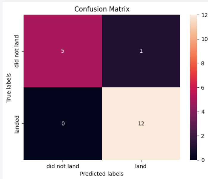
LogReg confusion matrix
